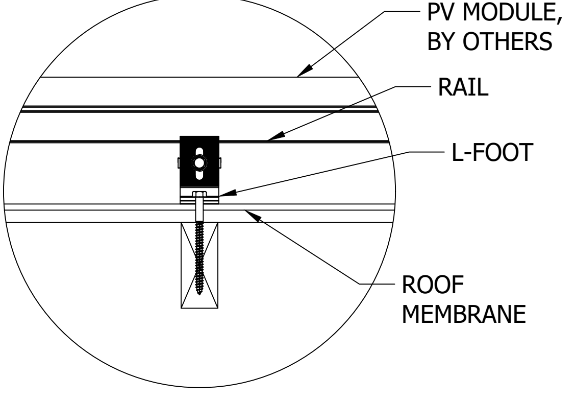
J GF-1 DETAIL FRONT Scale: 3"=1'-0"
