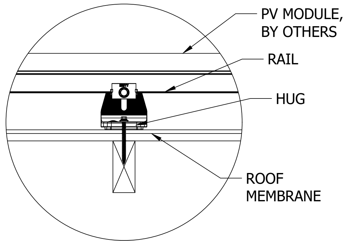
J HUG DETAIL FRONT Scale: 3"=1'-0"
