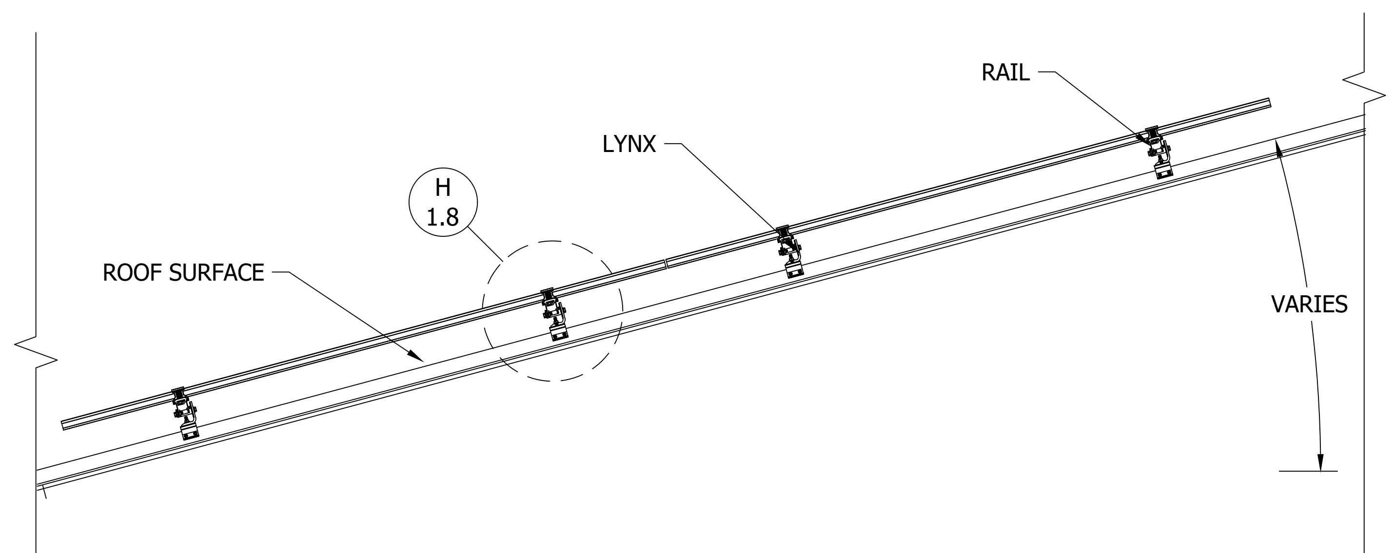
B SIDE VIEW, STANDING SEAM ASSEMBLY, PORTRAIT MODULE Scale: 1"=1'-0"
