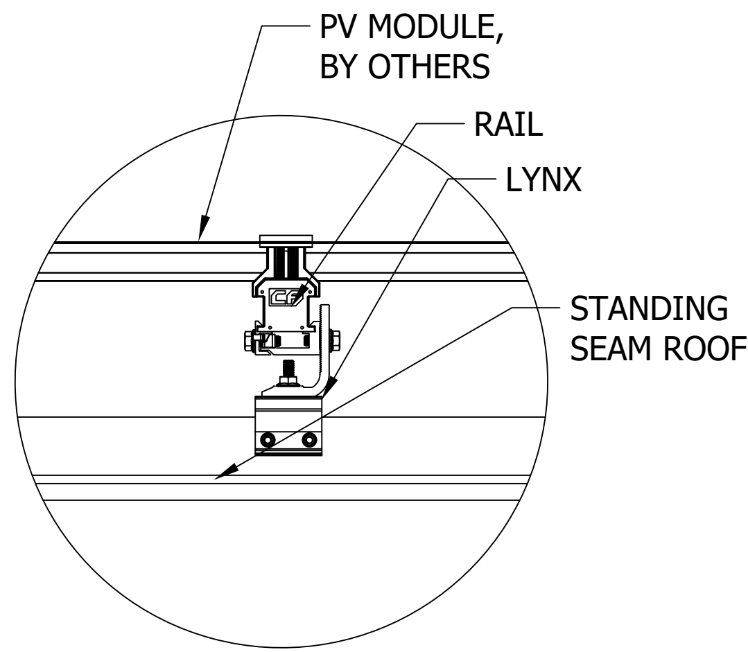
H CF SIMPLEBLOCK-U DETAIL SIDE Scale: 3"=1'-0"
