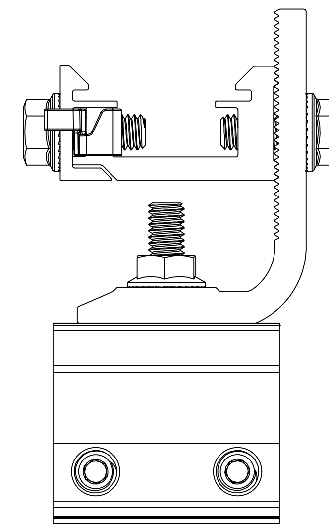
O ECOFASTEN CF SIMPLEBLOCK-U, FRONT VIEW
