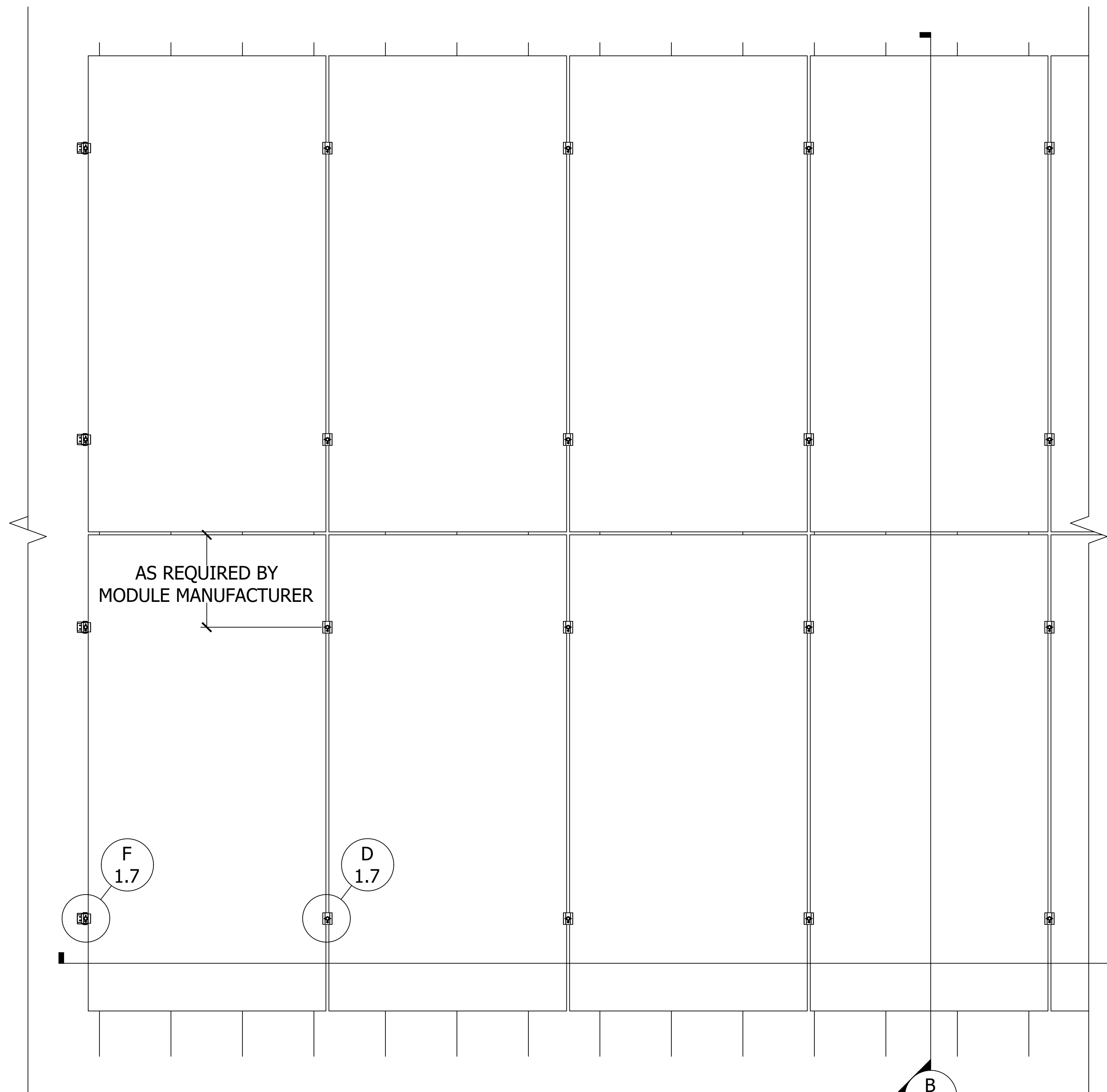
A PLAN VIEW, STANDING SEAM ASSEMBLY, PORTRAIT MODULE Scale: 1"=1'-0"
