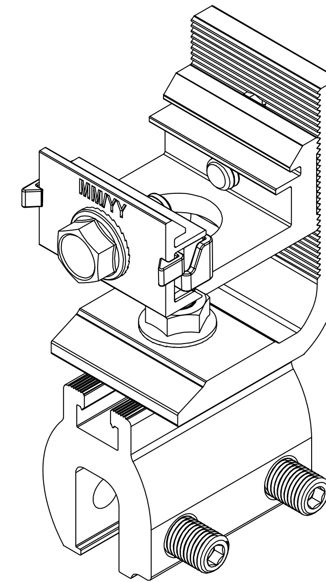
O ECOFASTEN CF SIMPLEBLOCK-U, FRONT VIEW
