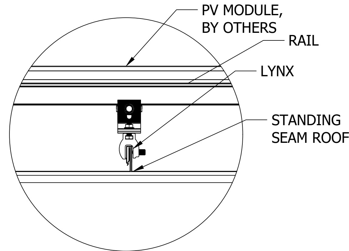
J CF SIMPLEBLOCK-U DETAIL FRONT Scale: 3"=1'-0"
