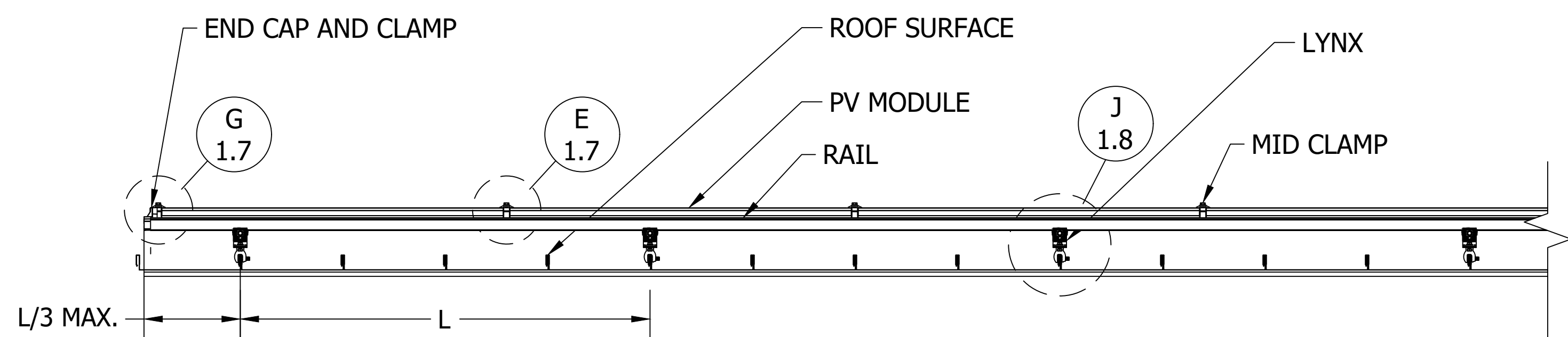
C FRONT VIEW, STANDING SEAM ASSEMBLY, PORTRAIT MODULE Scale: 1"=1'-0"
