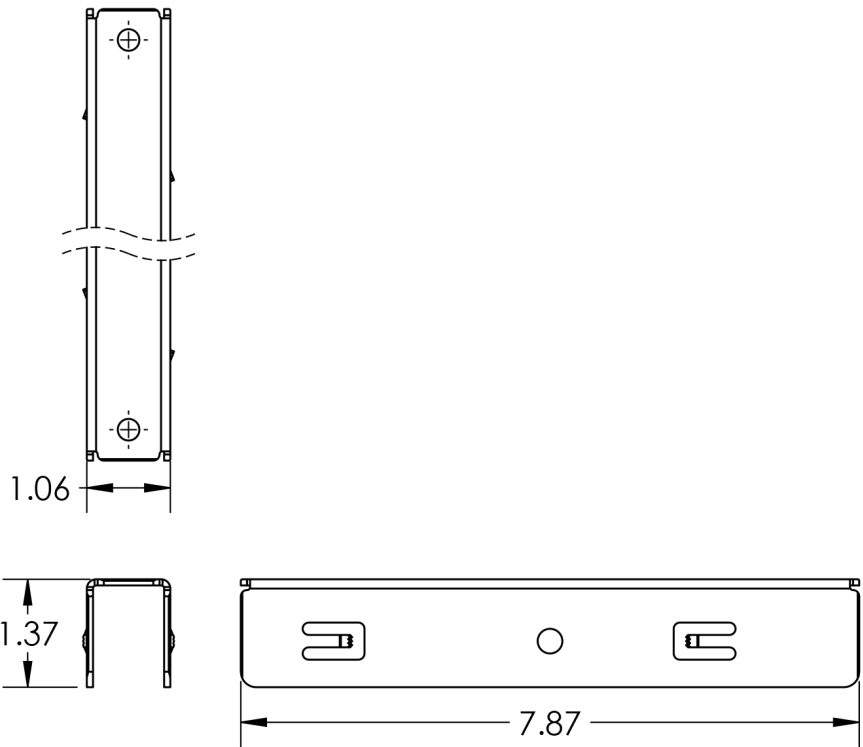
1) RAIL COUPLER
